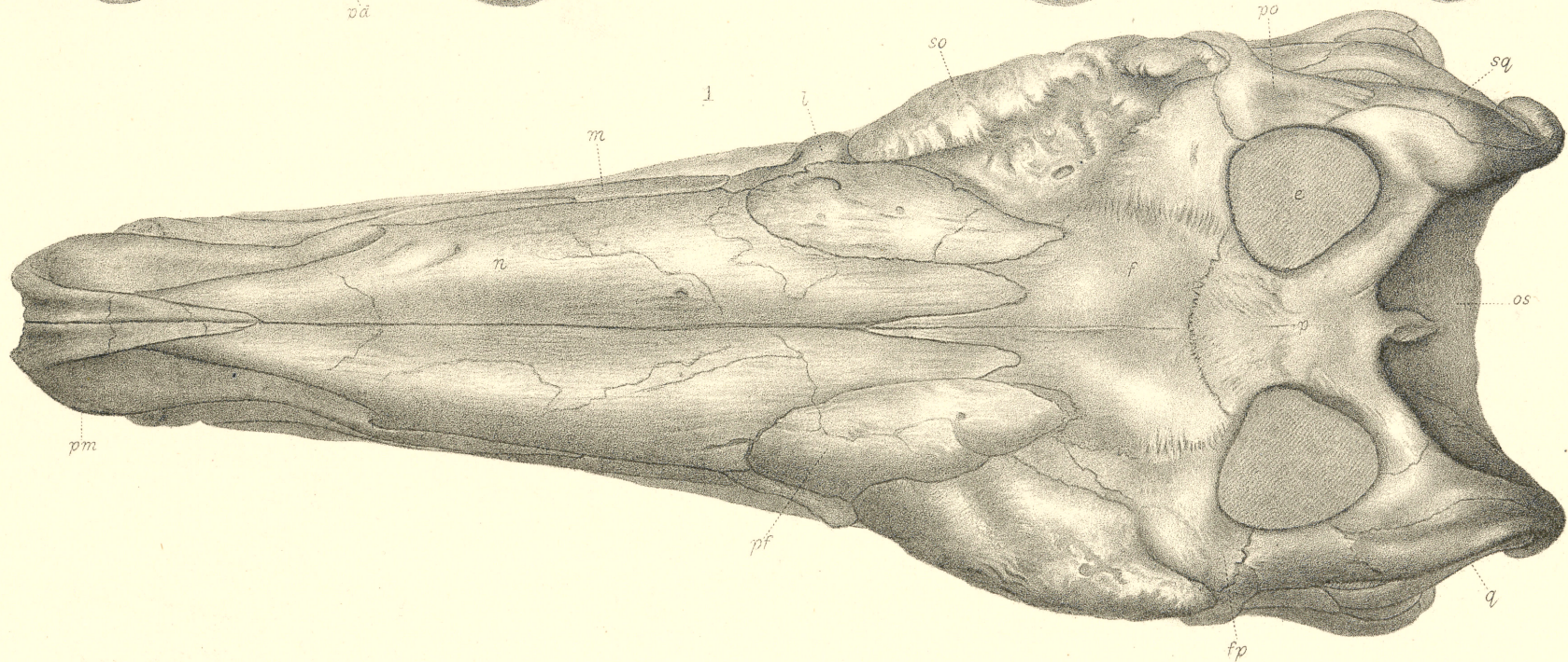
STEGOSAURUS STENOPS, Marsh. 1/2.
