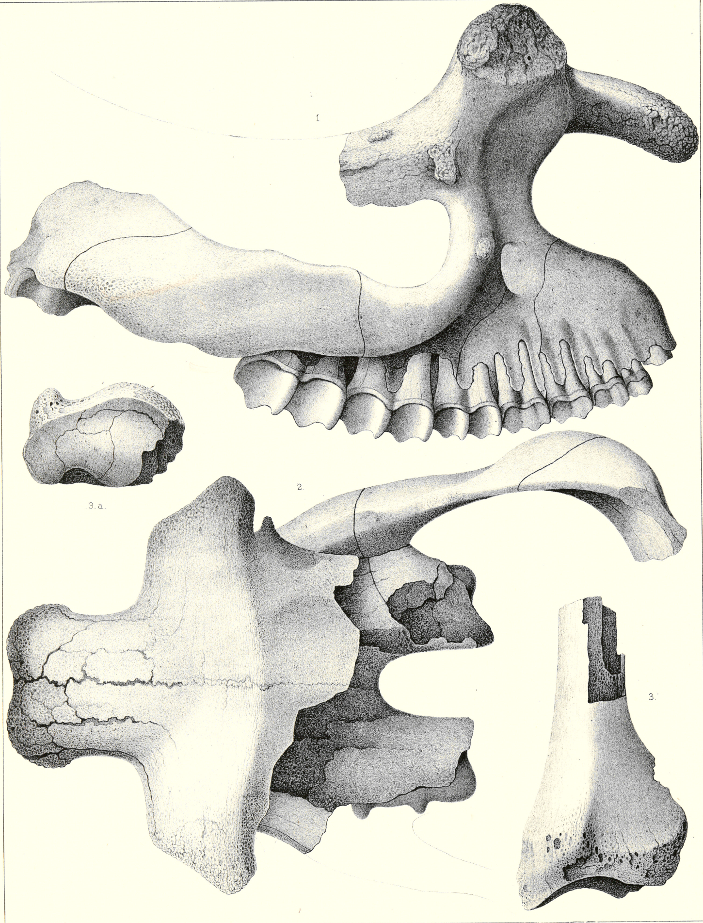
1 - 2. SYMBORODON TRIGONOCERAS \frac{1}{3}
